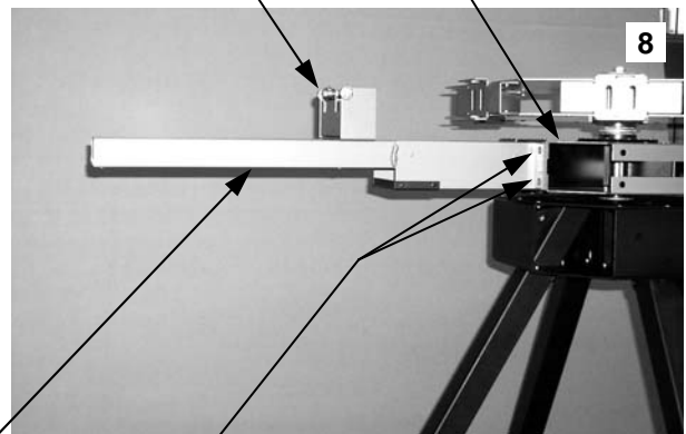
Rotor Arm (4) 3/8 bolts, lock washers, & hex nuts
