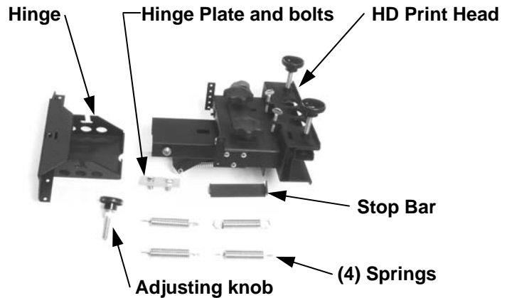
HD Print Head
